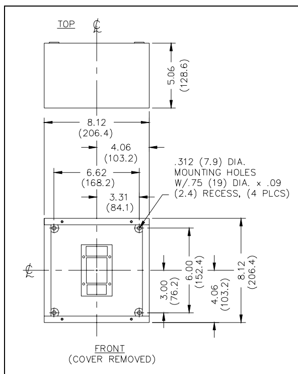
Figure 1. Mounting Details
